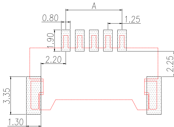
PCB LAYOUT
